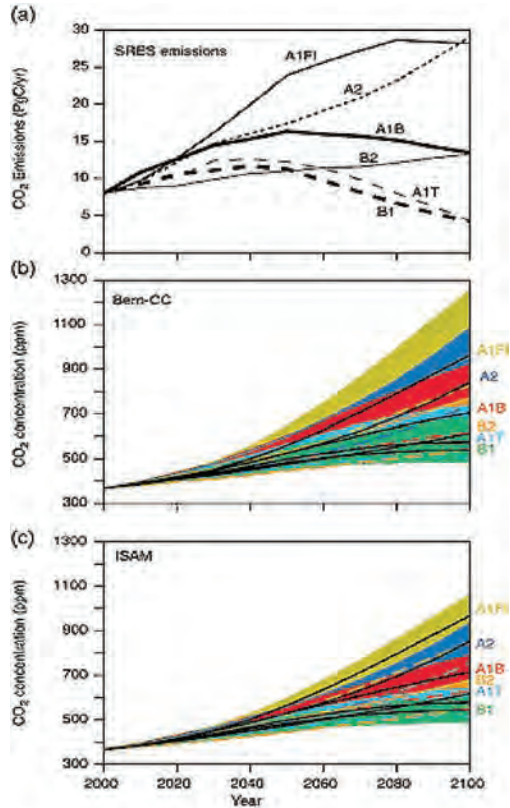
Figure 18. A possible range of carbon dioxide emissions and the resulting atmospheric changes. (IPCC WG1 2001, p. 222)
