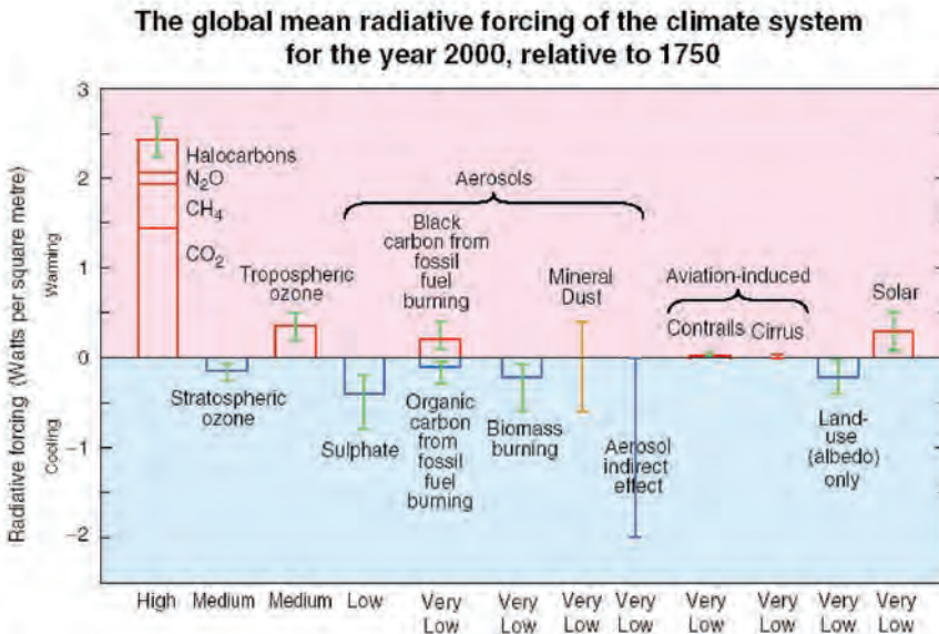
Figure 16. Many external factors force climate change. The error bars show ranges of uncertainty in radiative forcing (IPCC 2001, p. 37).
